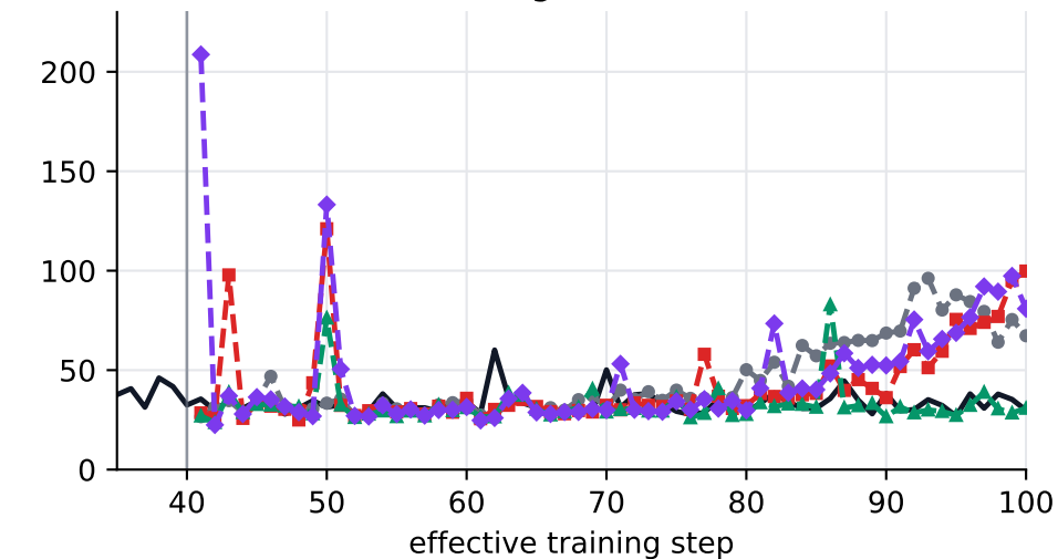
actor grad norm
