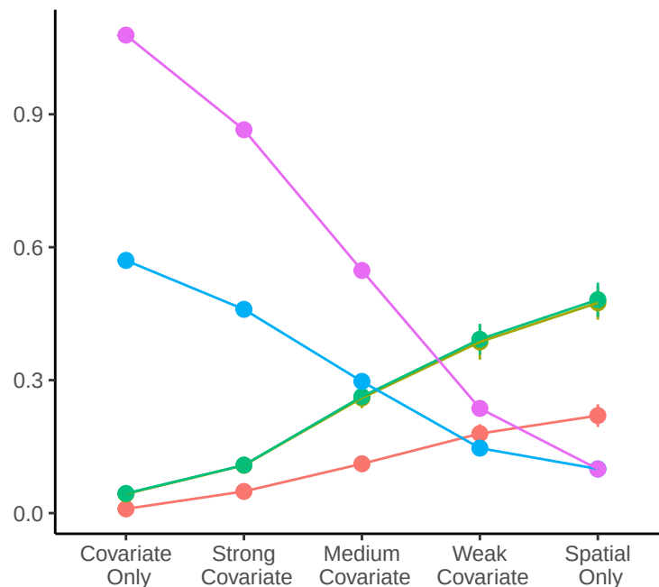
Interval Scores
