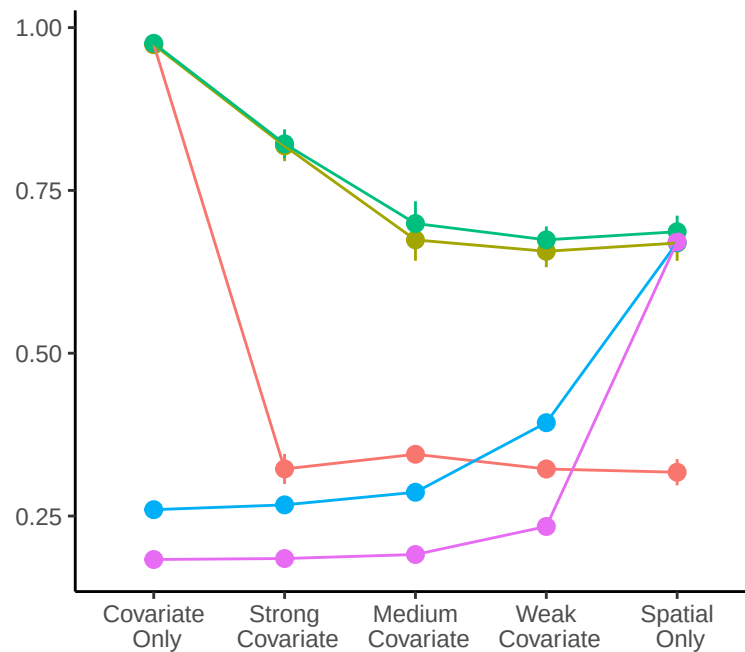
Coverage Rates
