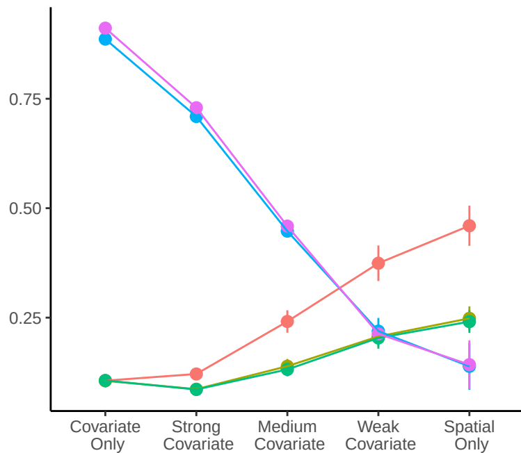
RMSE
