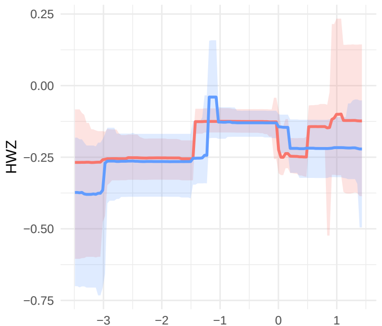
vegetation index
