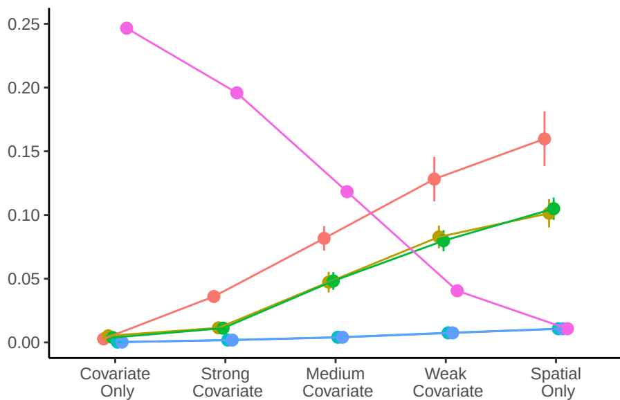
Interval Scores
