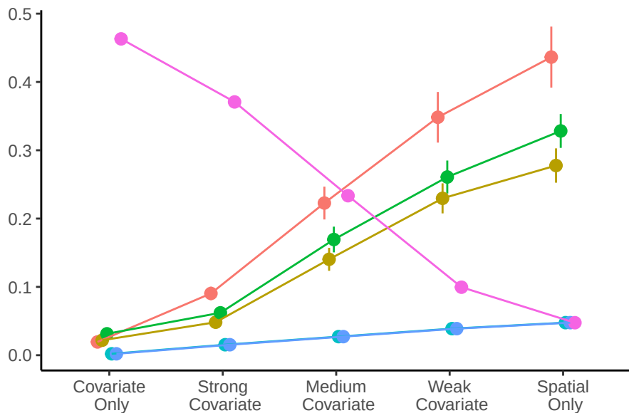
RMSE
