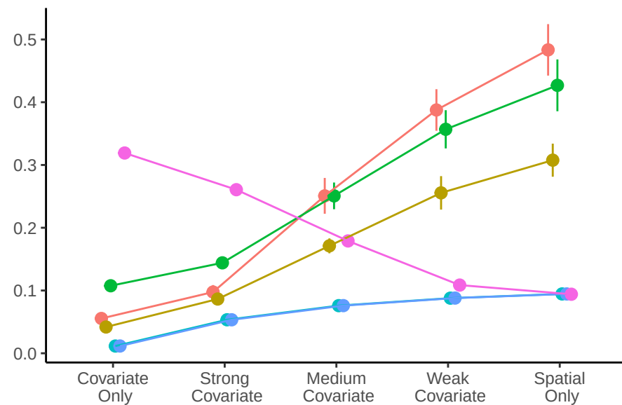
Interval Widths
