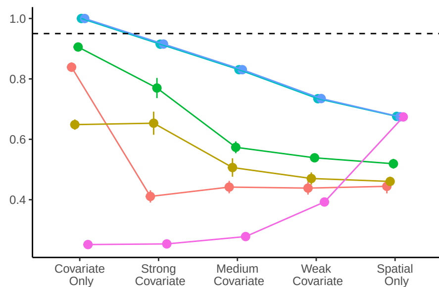
Coverage Rates
