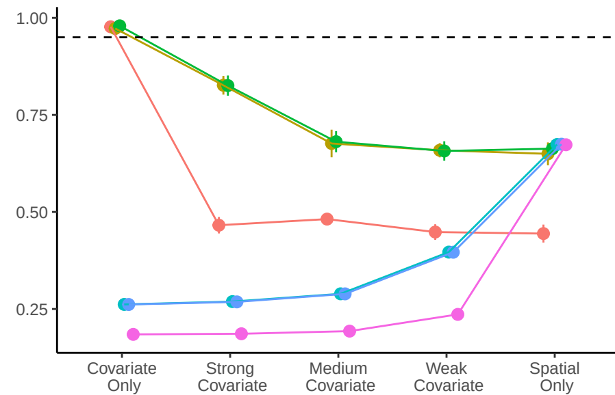
Coverage Rates
