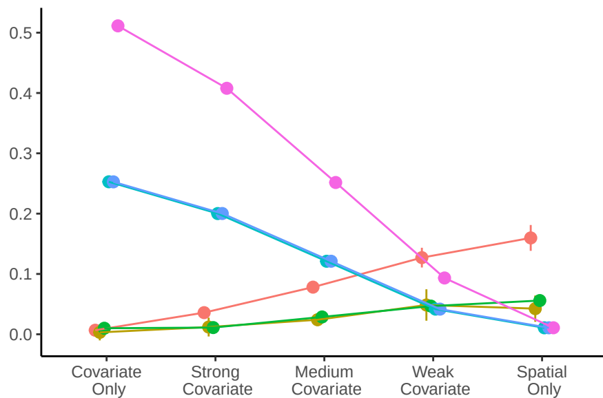
Interval Scores
