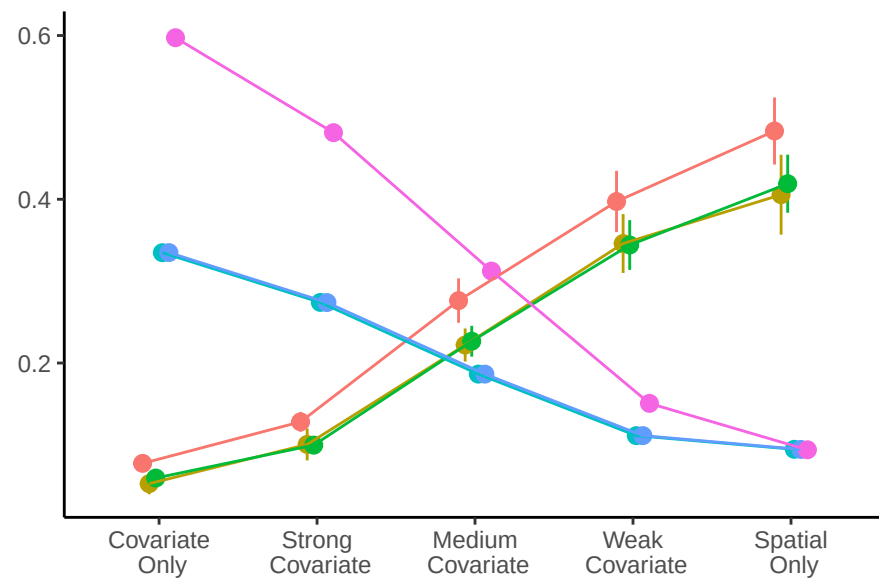
Interval Widths
