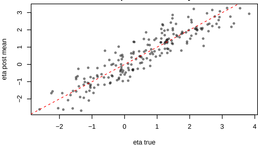
linear predictor recovery
