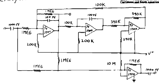
PEAK /NOTCH FILTER
