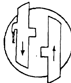
Outaway end view of lock Wafers may be spring or gravity operated
