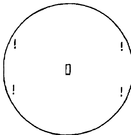
Outaway end view of lock Wafers may be spring or gravity operated
