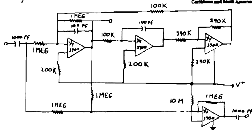
PEAK / NOTCH FILTER
