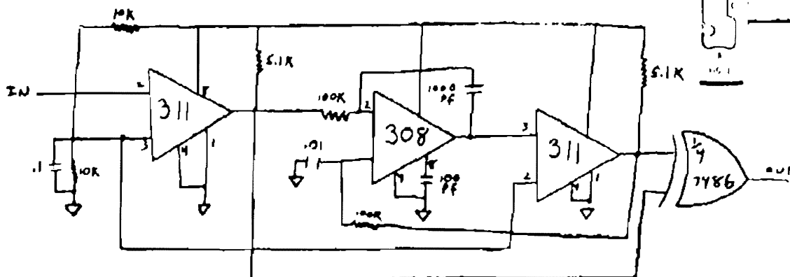
FREQUENCY DOUBLER
