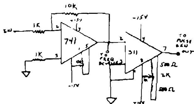
Product Detector Module
