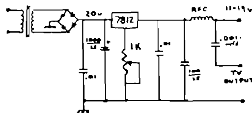
PS & TUNING UNIT
