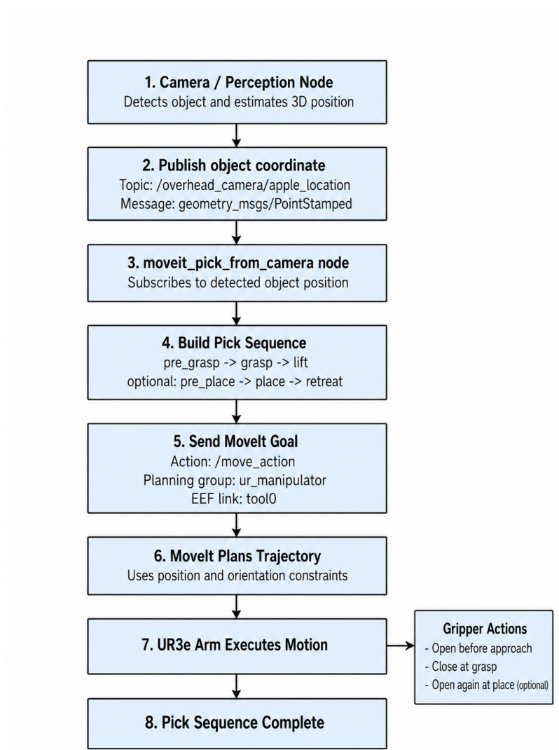
Figure 1: Pipeline of the MoveIt object pickup node
