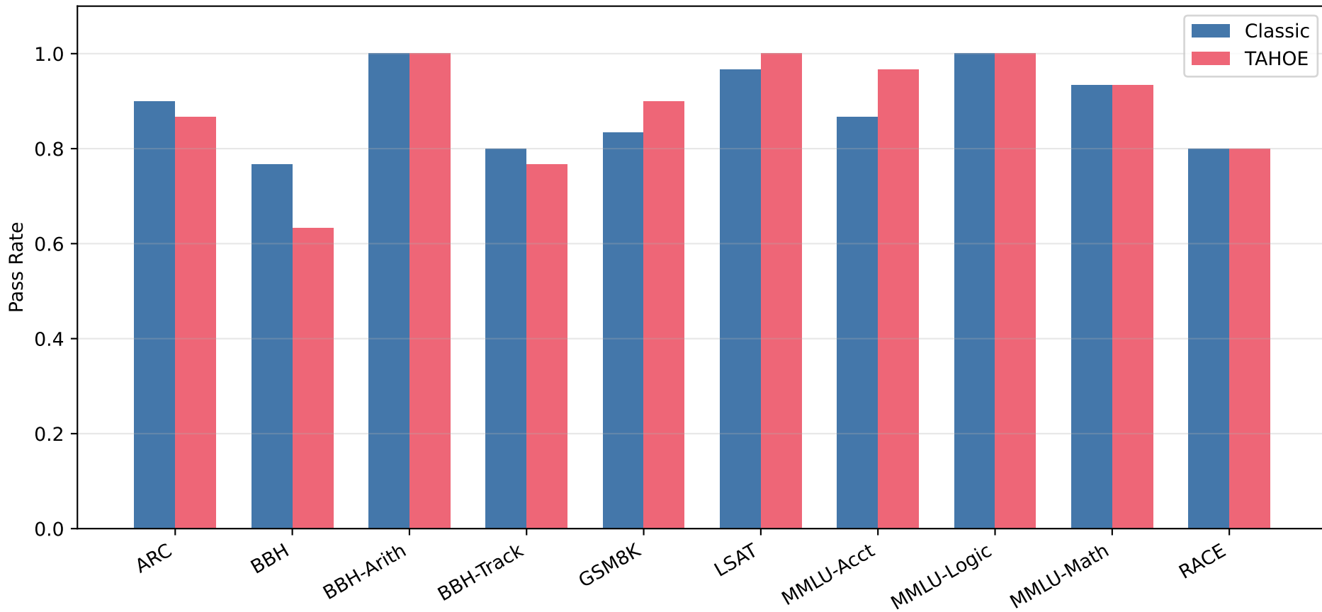
Figure 2: Pass Rate by Benchmark
