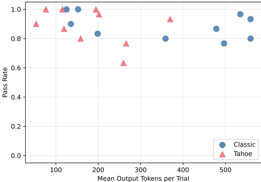
Figure 1: Quality vs Output Tokens
