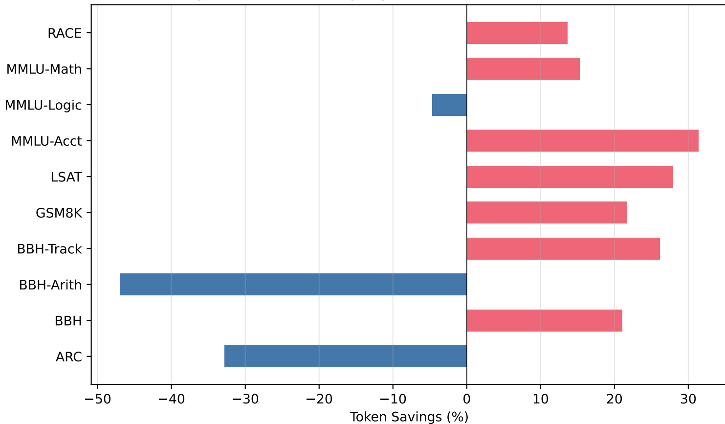
Figure 3: Token Savings by Benchmark (TAHOE vs Classic)
