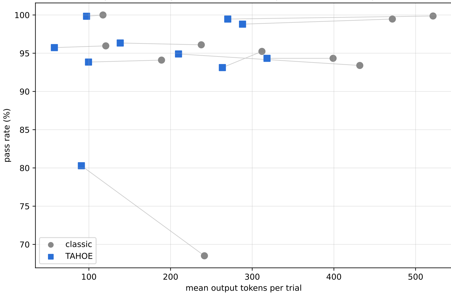
Quality vs reasoning tokens: TAHOE occupies the low-token quadrant
