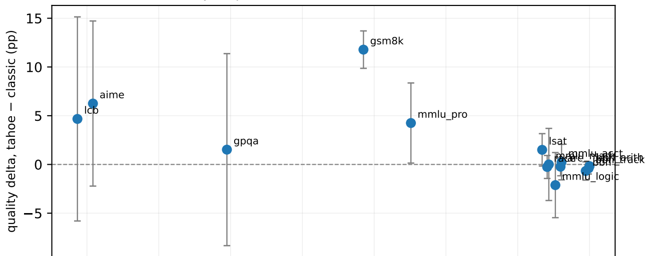
Difficulty response: GLM-5.3-Flash, tahoe-93 vs classic
