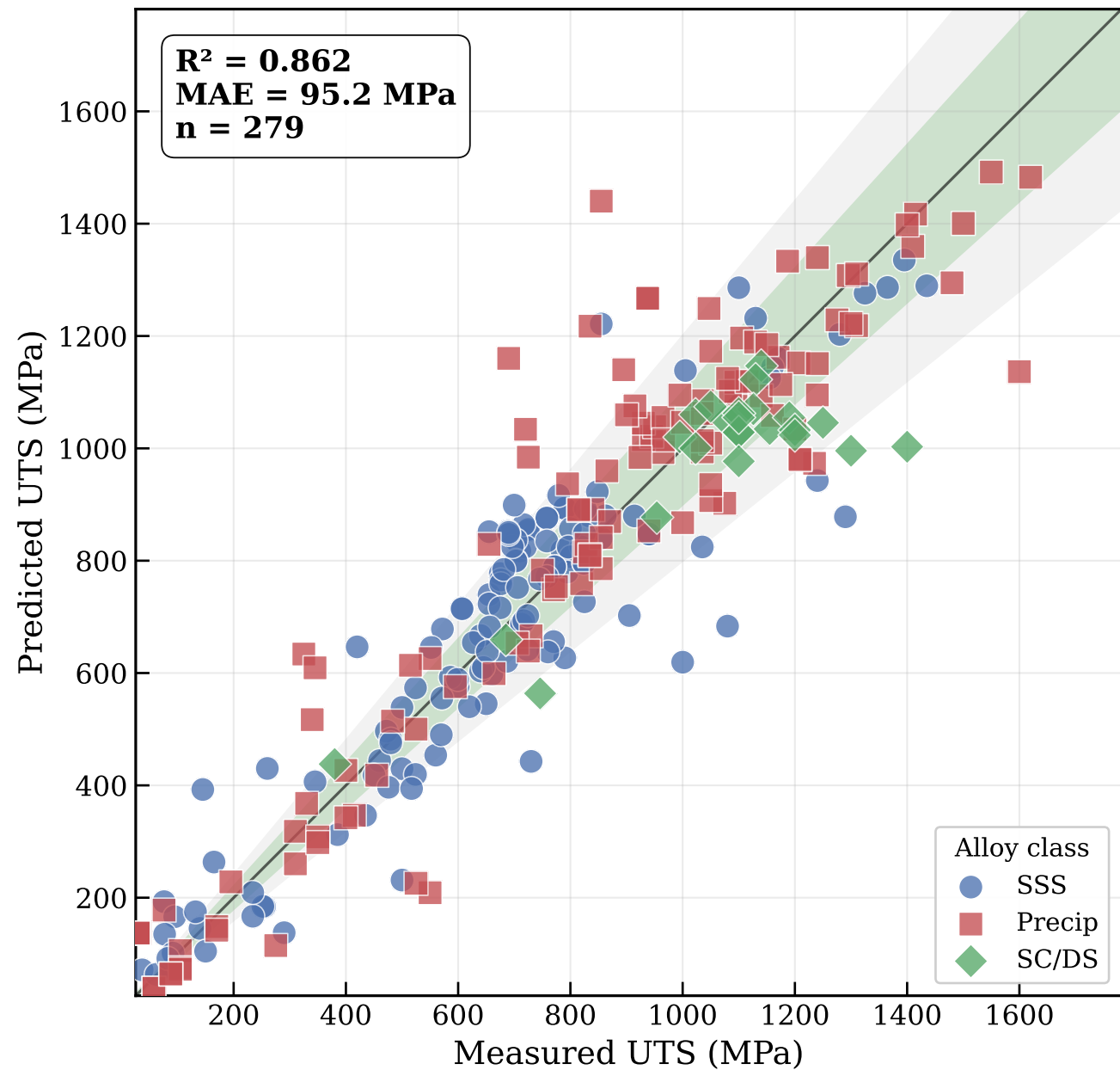
(b) Ultimate tensile strength
