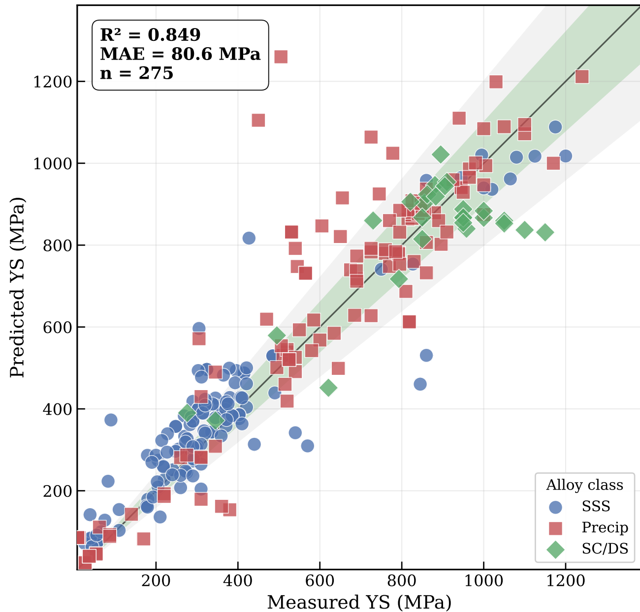
(a) Yield strength
