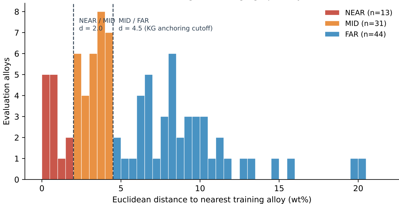
Compositional distance from the 88 evaluation alloys to the 77 training / knowledge-graph alloys
