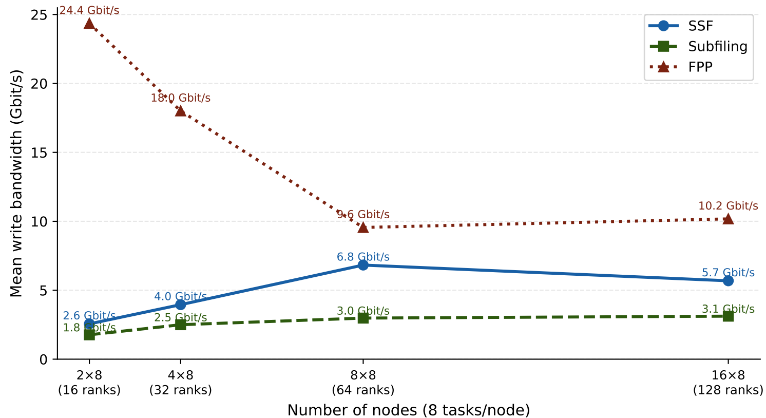
Write bandwidth vs. node count — SSF, Subfiling, FPP (8 tasks/node, sc=8, BeegFS/Plafrim)
