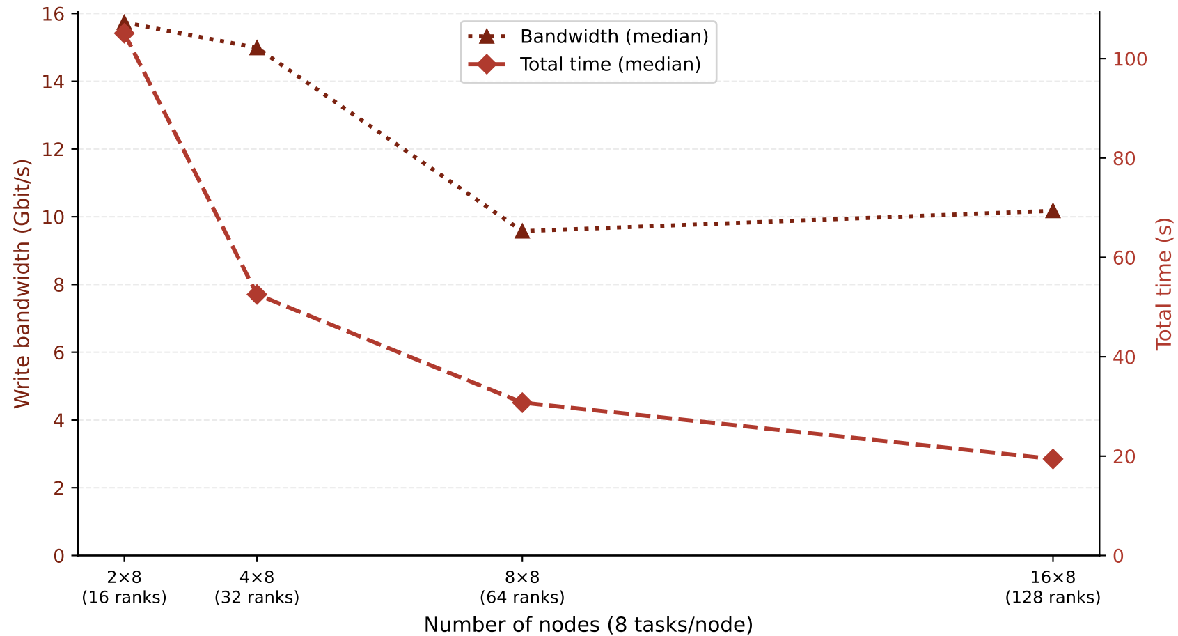
Bandwidth vs. total time — node count (FPP strategy, 8 tasks/node, median of n=3 runs)
