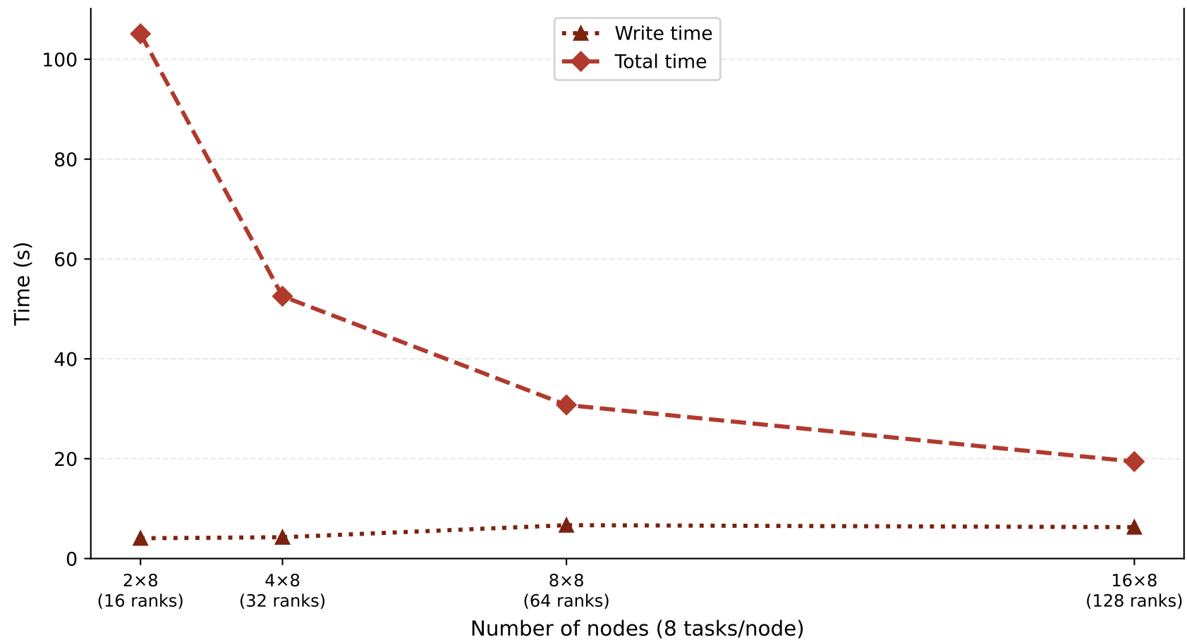
Write time vs. total time — node count (FPP strategy, 8 tasks/node)
