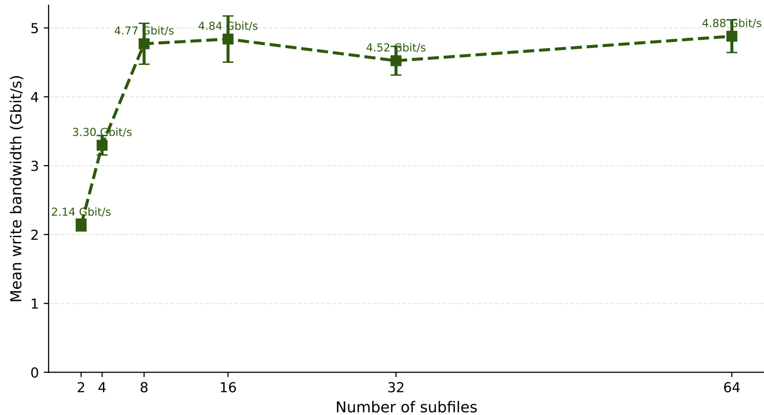
Write bandwidth vs. subfile count (Subfilng strategy, 16 nodes \times 8 tasks/node)
