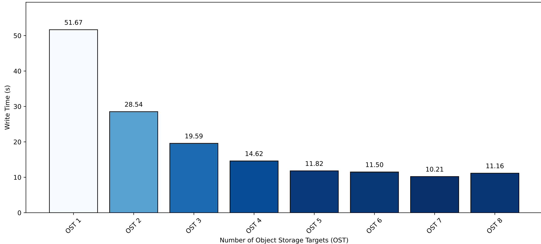
Impact of OST count on write time MPI configuration: 16 nodes \times 8 processes/node, 512 KB chunk size
