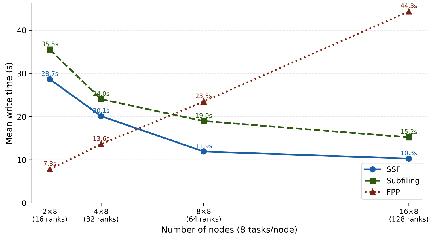
Write time vs. node count — SSF, Subfiling, FPP (8 tasks/node, sc=8, BeegFS/Plafrim)
