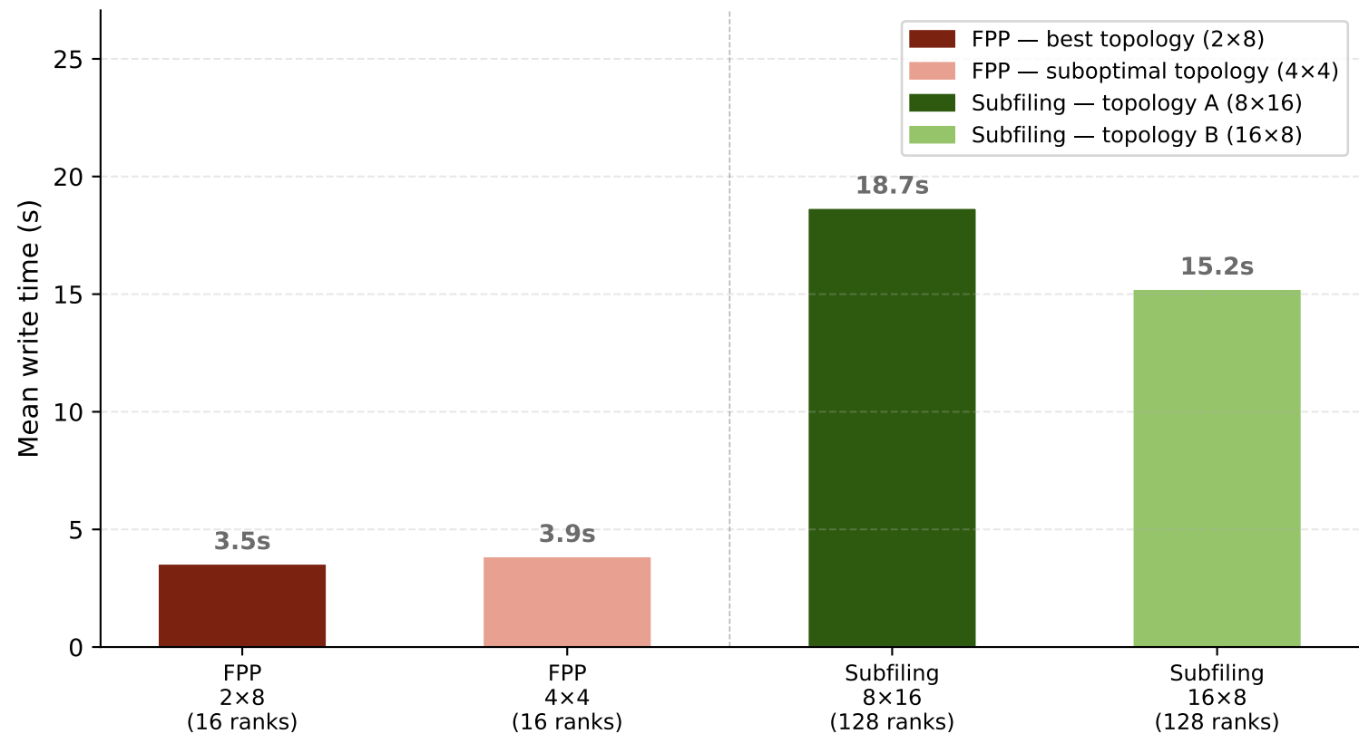
MPI topology impact at equal rank count (same data volume, sc=8, BeegFS/Plafrim)
