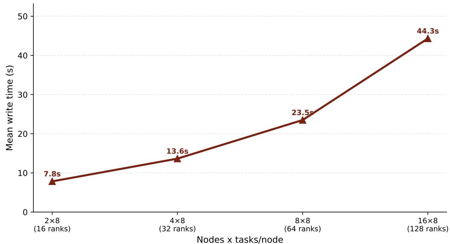
FPP: write time degradation with node count (8 tasks/node, sc=8, BeegFS/Plafrim)
