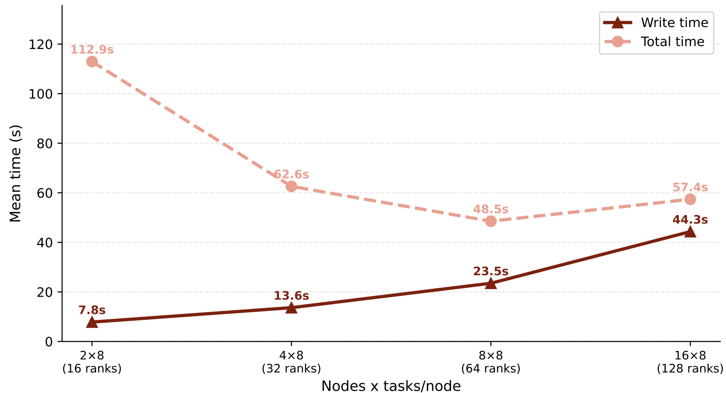
FPP: write time vs. total time degradation with node count (8 tasks/node, sc=8, BeegFS/Plafrim)
