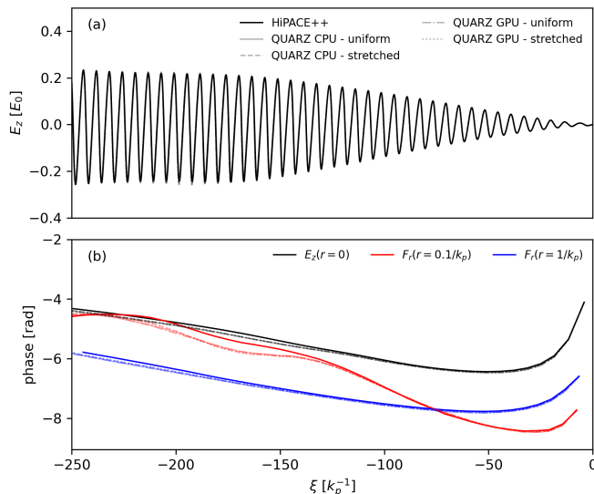
FIG. 6. Self-modulation of the AWAKE proton bunch after 6 m of plasma: QUARZ on uniform (3840 cells) and stretched (403 cells) radial grids, on CPUs and GPUs, compared with HiPACE++. (a) E_z on the axis, with the head of the bunch at \xi = 0 . (b) Phase of E_z(r=0) and of the transverse force F_r = E_r - B_\theta at r = 0.1 and 1/k_p , from the zero crossings of the fields. Saturated lines: HiPACE++; light lines: the four QUARZ runs.
