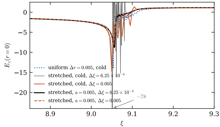
(a) on-axis field at the bubble closure
