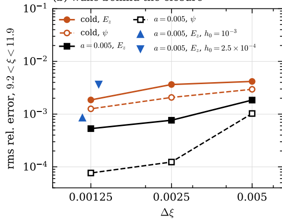
(b) wake behind the closure
