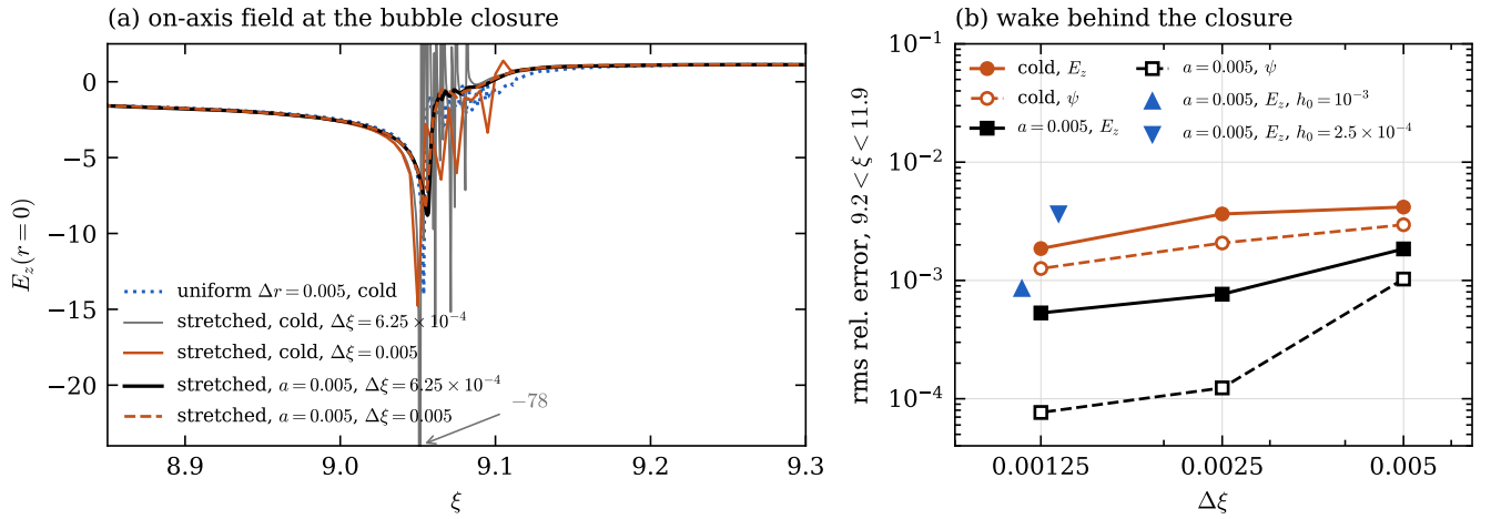
FIG. 5. Bubble closure in the pinched-witness case of Fig. 2, with the box extended to \xi = 12 (single quasi-static solve). (a) E_z on the axis at the closure: uniform grid \Delta r = 0.005 ; stretched grid ( h_0 = 5 \times 10^{-4} ) with a cold plasma and with smoothing of the plasma sources, Eq. (14), a = 0.005 . The cold spike reaches -78 at \Delta \xi = 6.25 \times 10^{-4} . (b) Rms relative error of E_z(0) and \psi(0) behind the closure ( 9.2 < \xi < 11.9 ) versus \Delta \xi , with respect to \Delta \xi = 6.25 \times 10^{-4} of the same model. Triangles: a = 0.005 with axis cells 10^{-3} and 2.5 \times 10^{-4} ( \Delta \xi = 0.00125 ).
