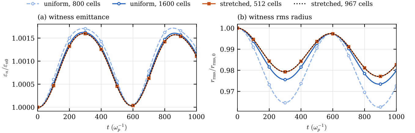
FIG. 4. Evolution of the pinched witness of Fig. 2 behind a rigid driver, with mobile hydrogen ions, on two uniform and two stretched grids ( \Delta t = 10 , 2 \times 10^5 witness particles). (a) Normalized emittance, (b) rms radius, both relative to their initial values. The 512-cell stretched grid coincides with the 967-cell one; the uniform grids overestimate the envelope oscillation.
