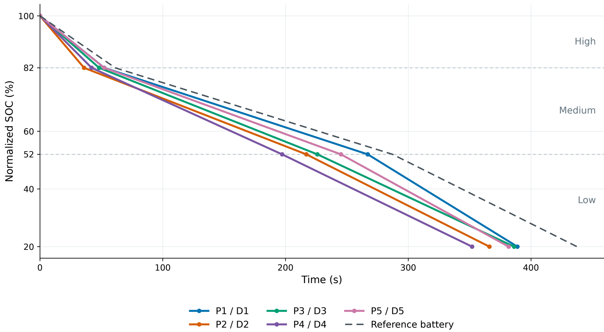
Three-stage configuration discharge curves on the existing reference-battery scale Diamond · 50 cm · Headwind · Level 2
