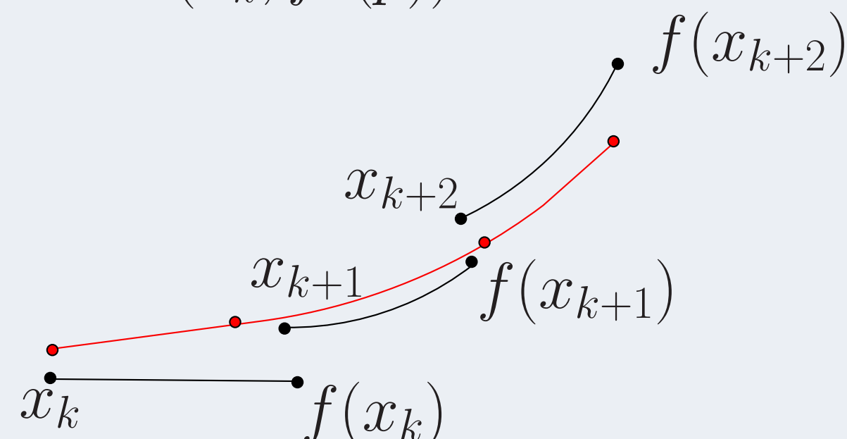
Figure: Example when POTP holds: black denotes a pseudotrajectory, red denotes an exact trajectory.
