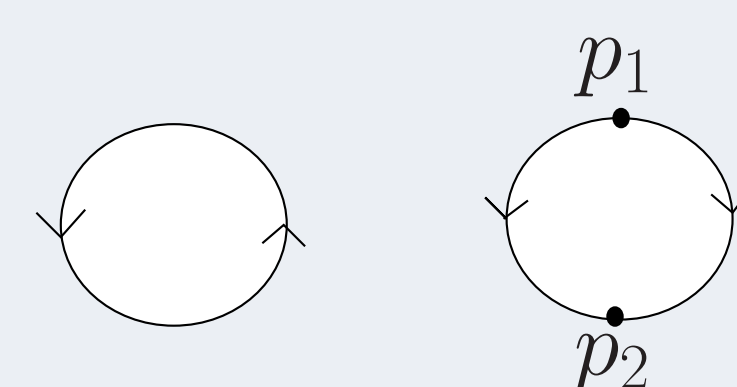
Figure: Diffeomorphisms g_0 and g_1 .
