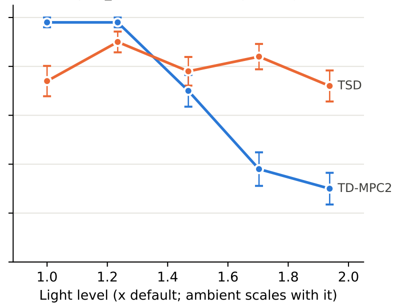
push_cube — Simulation planning
