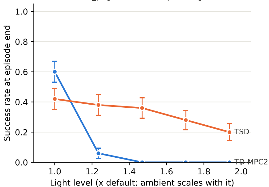
lift_peg — Real-time planning
