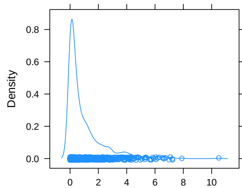
(b) Densityplot
