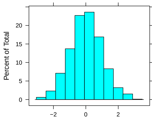
(a) Histogram
