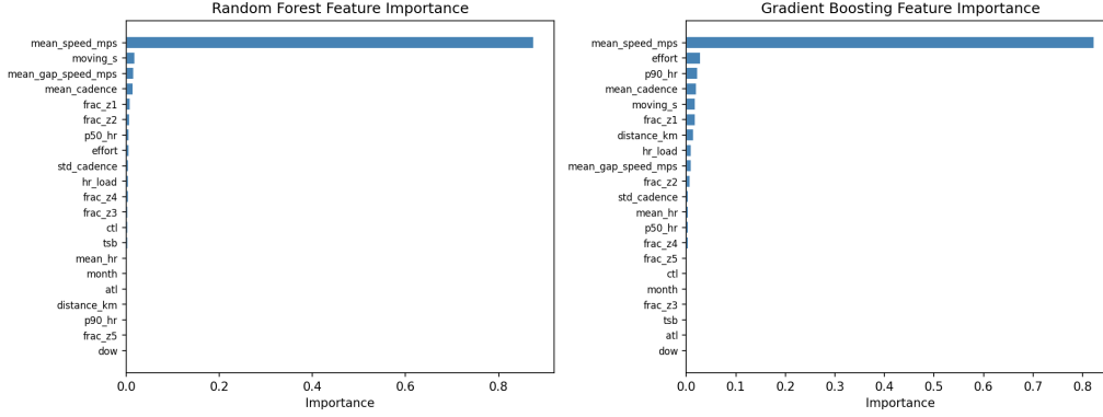
Figure 7: Feature Importances for Random Forest and Gradient Boosted Regression (Mean Decrease in Impurity, Normalised to Sum to 1). Mean speed dominates; moving time, cadence, and effort fraction are the next most informative features.
