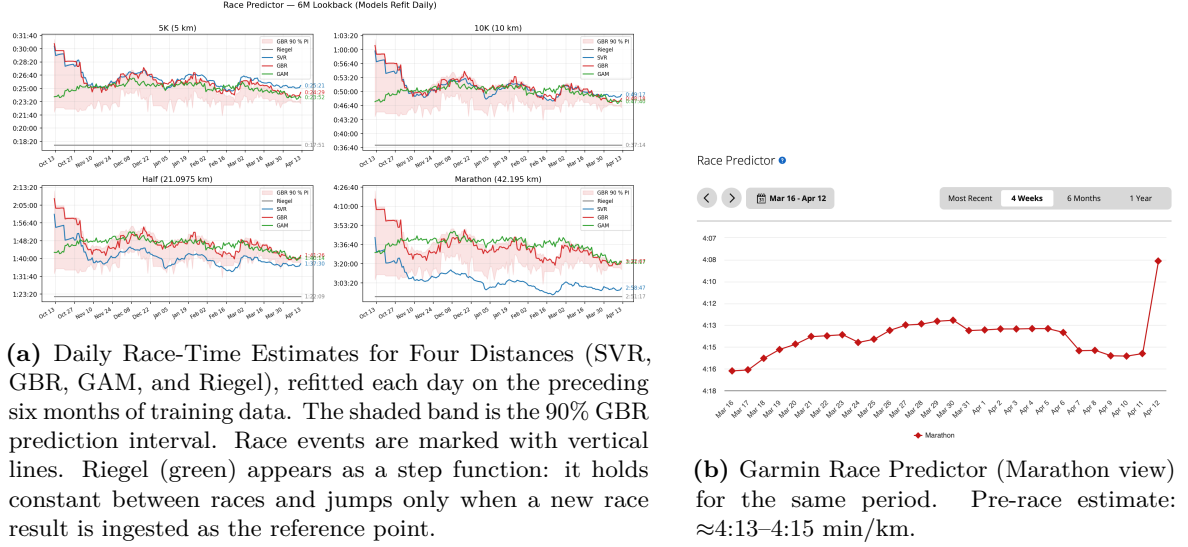
Figure 8: Comparison of the Pipeline’s Daily SVR Predictor (a) and the Garmin Race Predictor (b) for the 2026 Milano Marathon Build-Up. Both converge on a sub-3:00 estimate during the taper window.
