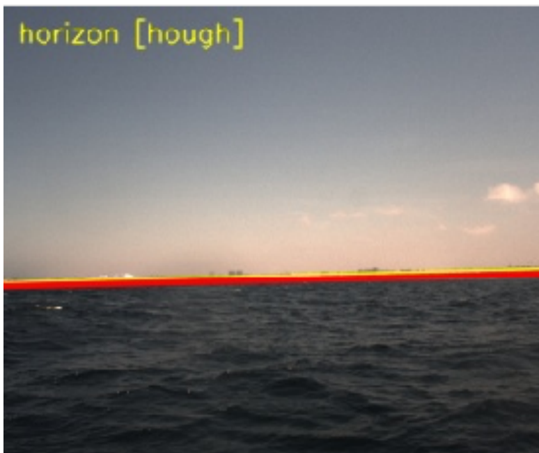
Figure 5: Sky/horizon masking applied by the shared pre-processing stage. Pixels above the detected horizon line (shown in red) are excluded from disparity estimation and point-cloud reconstruction, preventing sky matches from corrupting the sea-surface output.
