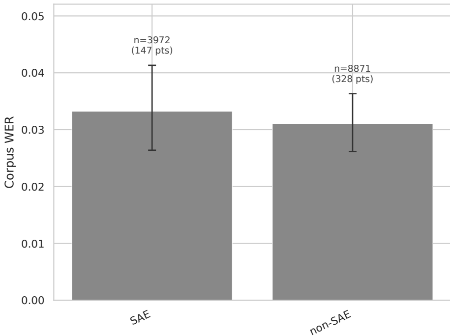
accent_simplified — Gemini self-transcribe — WER
