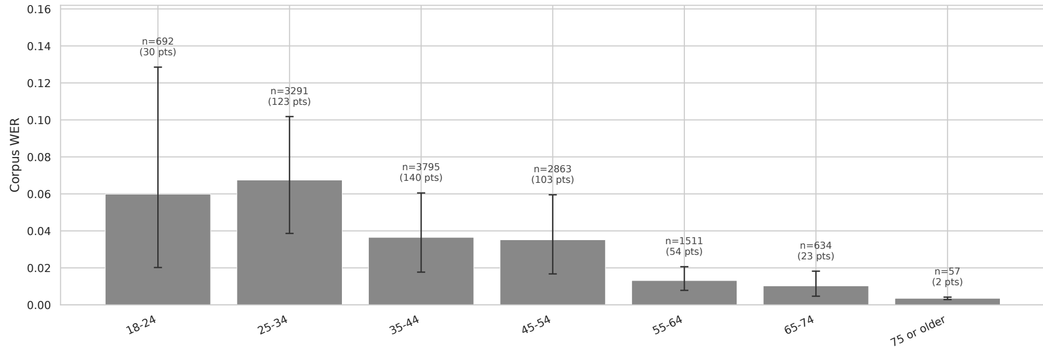
age — Whisper-1 — WER
