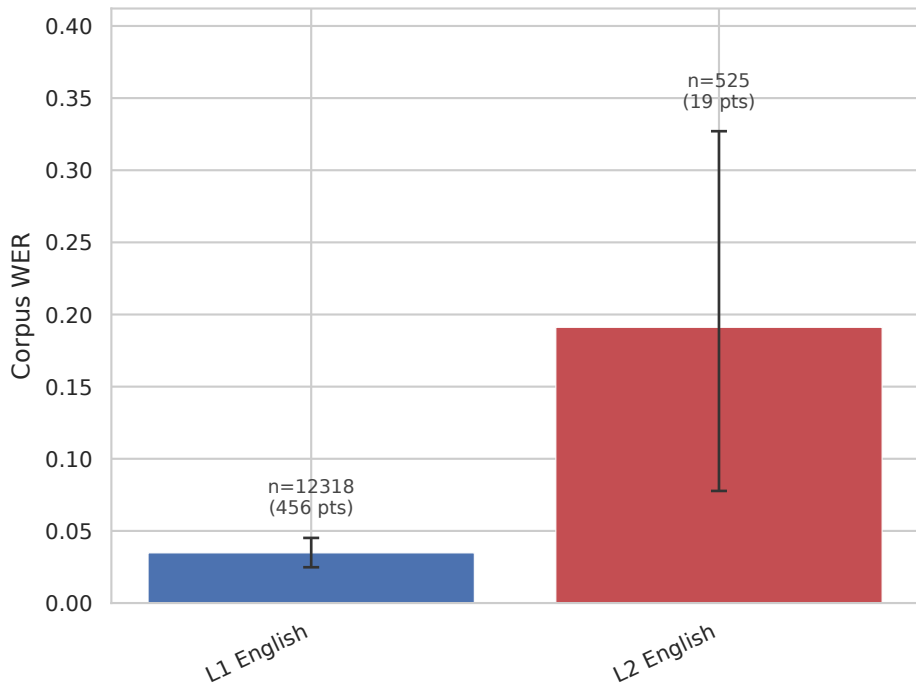
english_I1I2 — Whisper-1 — WER
