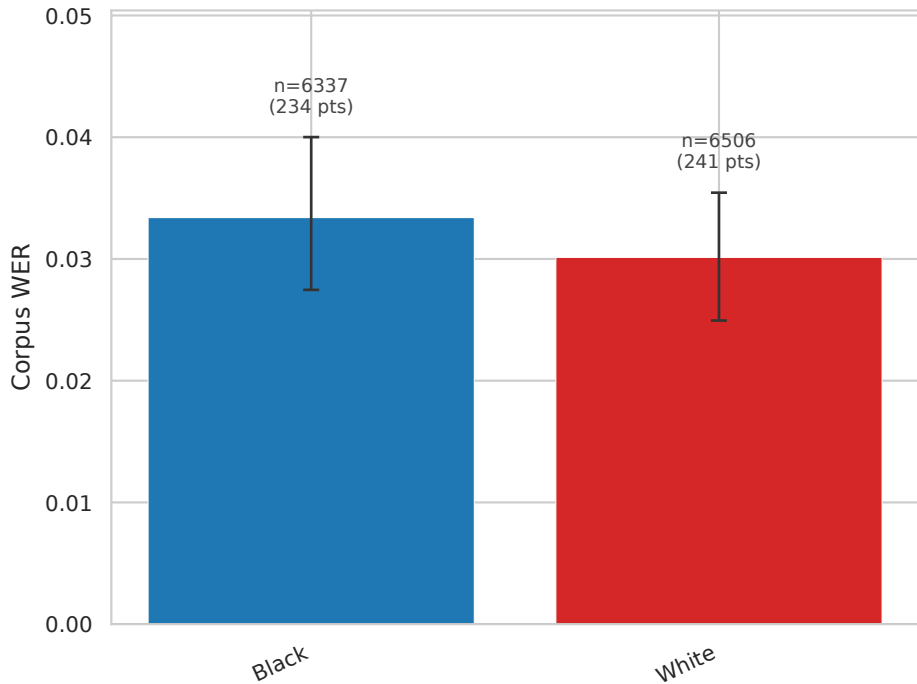
race — Gemini self-transcribe — WER
