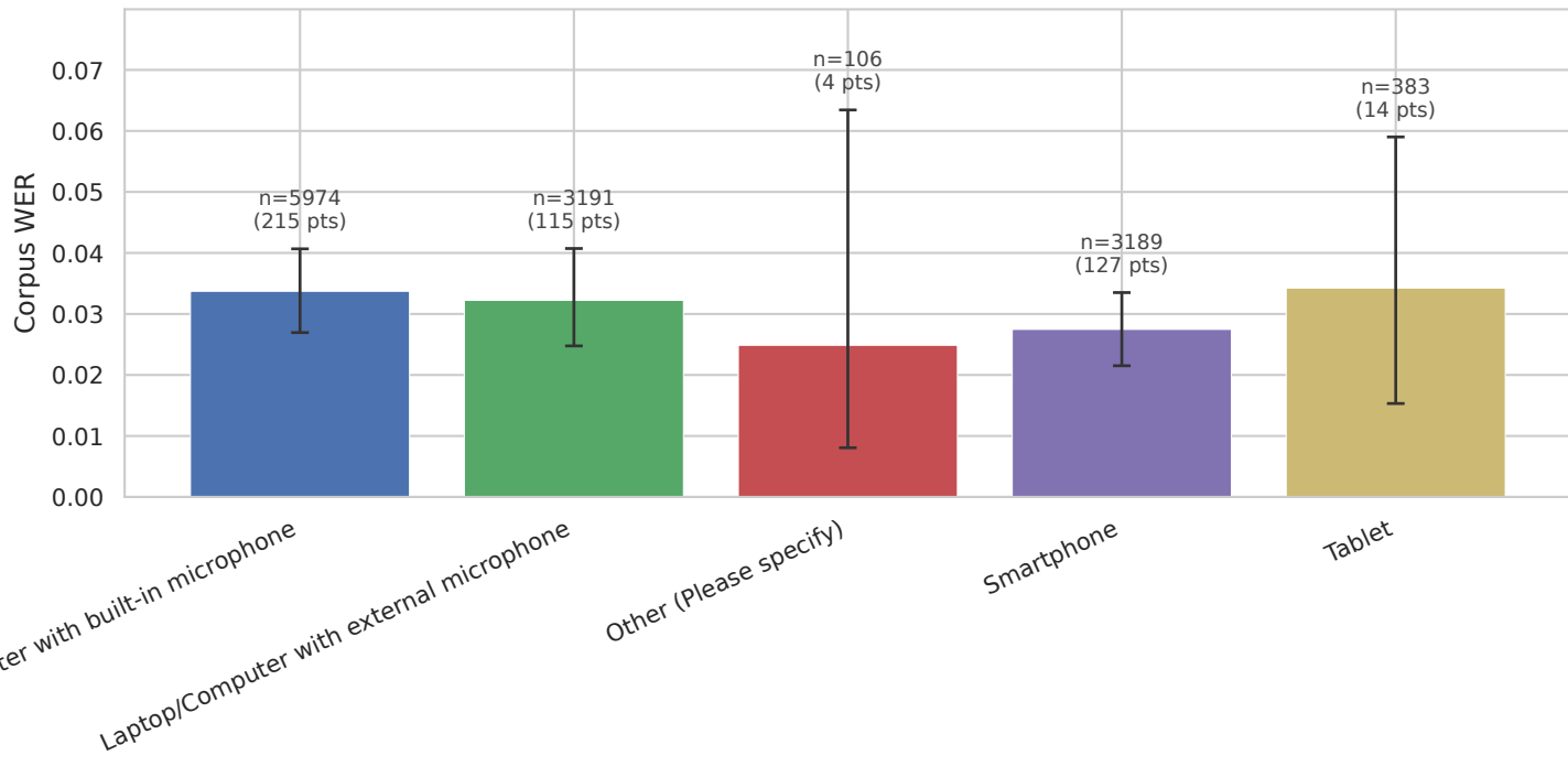
recording_device — Gemini self-transcribe — WER
