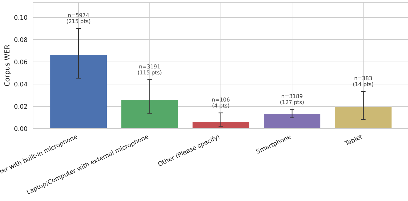
recording_device — Whisper-1 — WER
