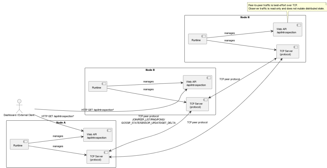
Figure 13: Deployment view of a multi-node cluster with peer TCP channels and read-only observer access.
