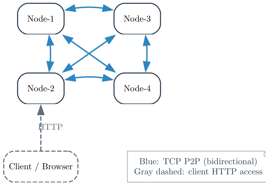
Figure 3: Infrastructure-level node connectivity in the base full-mesh deployment.
