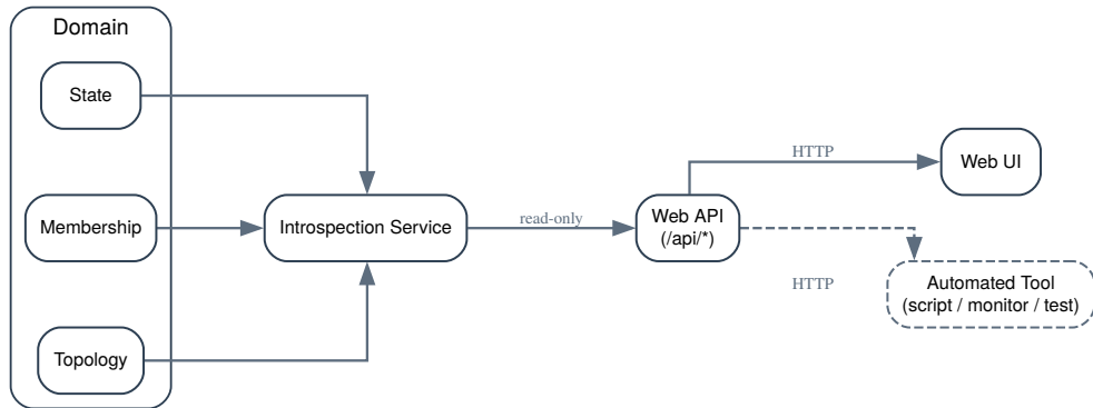
Figure 3: Observability architecture: introspection and read-only API exposure path.
