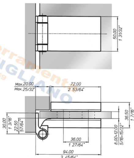
GAHA1ST6D Braccio Normale Regular Arm
