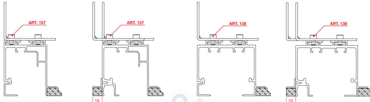
WALL / PARETE
