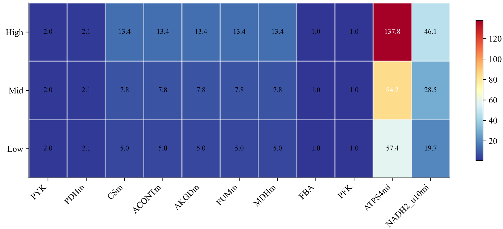
Recon3D Pathway Fluxes by Condition
