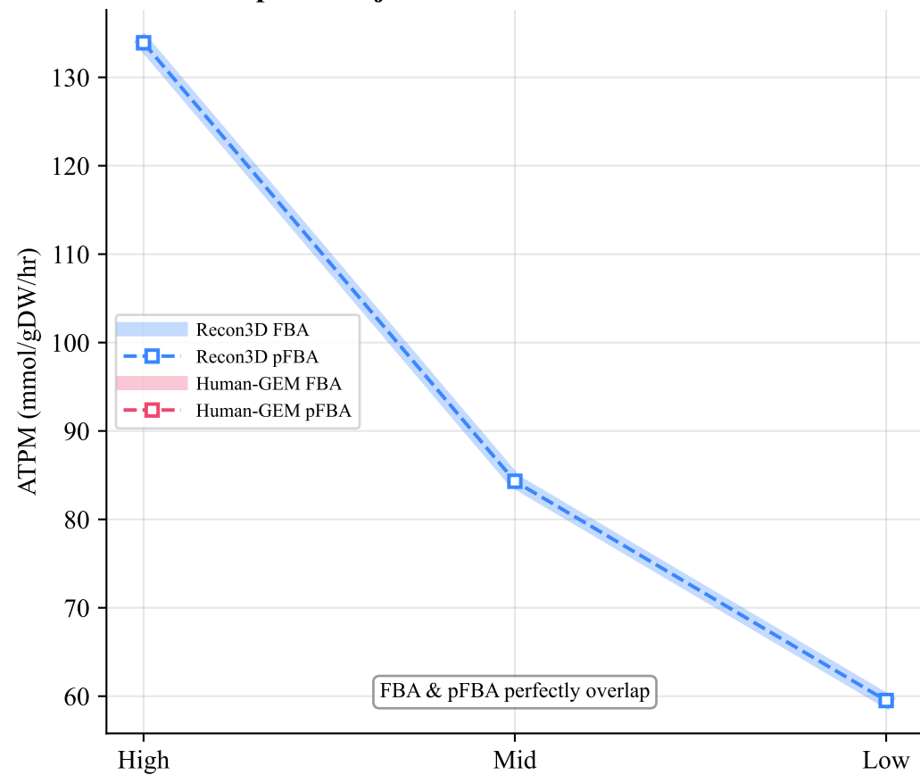
A FBA vs pFBA objective
