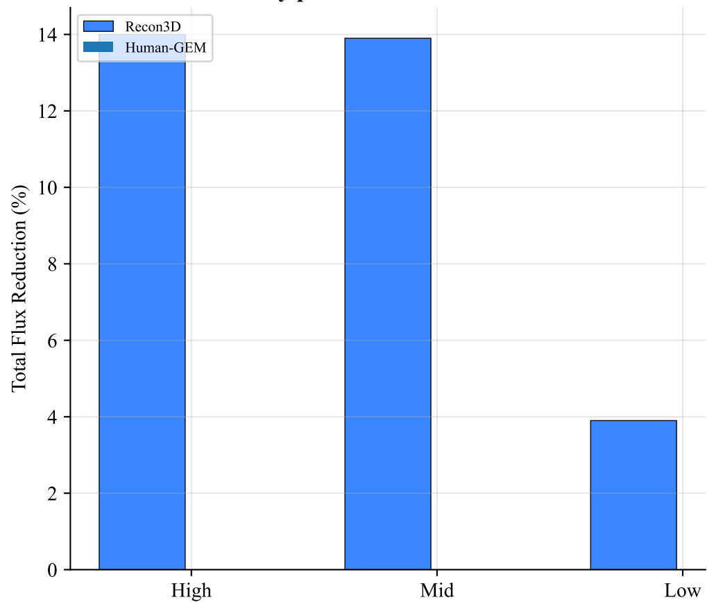
B Flux reduction by pFBA
