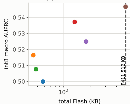
(c) int8 AUPRC vs Flash
