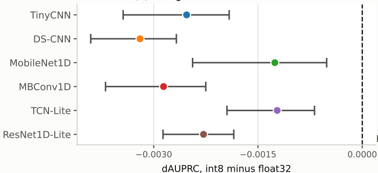
(a) change in macro AUPRC after int8
