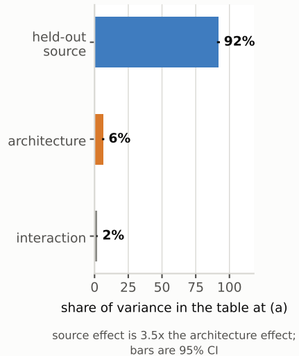
(c) what decides external AUPRC
