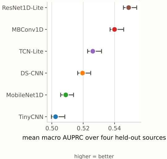
(b) mean AUPRC, record-level bootstrap 95% CI
