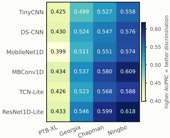
(a) macro AUPRC by held-out source
