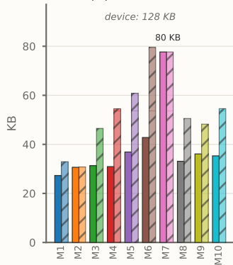
(B) Peak SRAM
