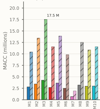
(C) Arithmetic cost
