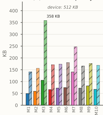
(A) Flash occupancy
